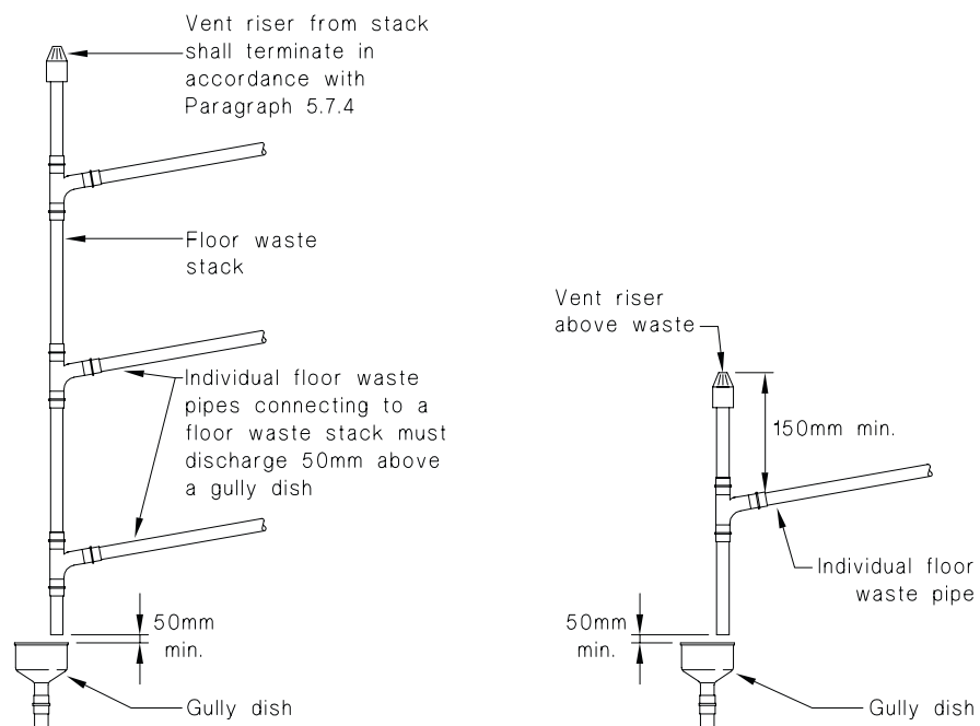
(a) Multiple floor waste pipes connecting to floor waste stack
