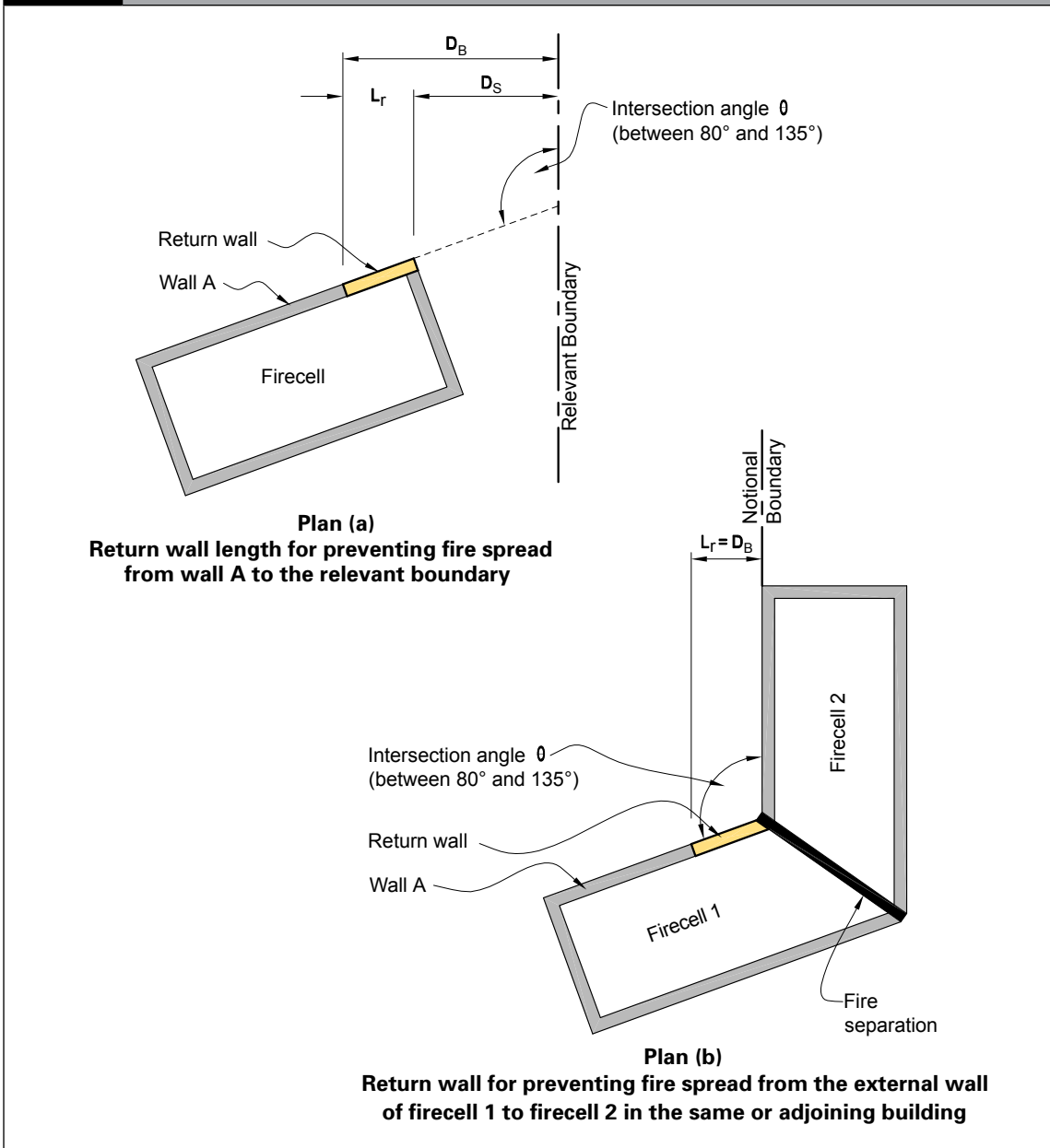
Figure C5 Method 4 – Return walls on external walls having an intersection angle of between 80° and 135° with the relevant boundary or notional boundary
