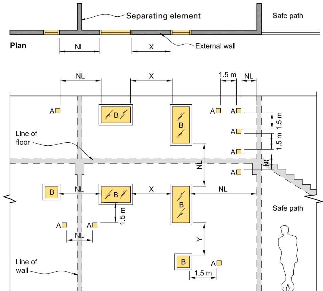
Figure C2 Method 1 – Permitted small unprotected areas and fire resisting glazing Paragraph C2.1.4
