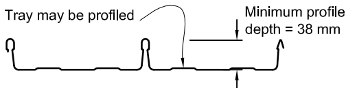
Trough Profile
