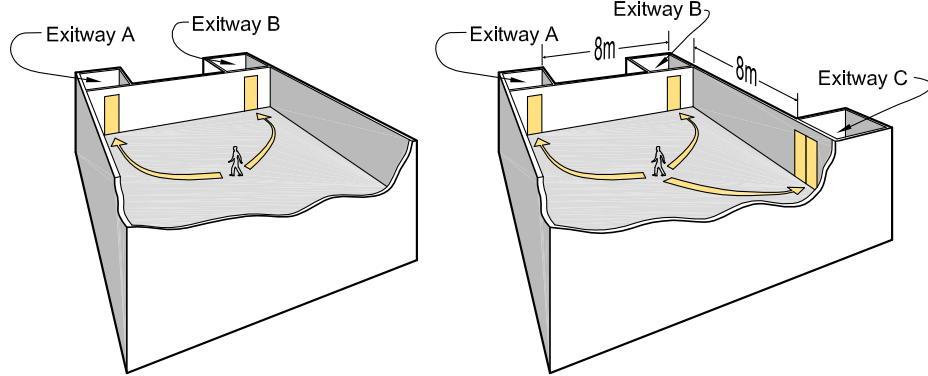
Figure 3.3 Exitway widths in unsprinklered firecells Paragraph 3.3.2 d)
