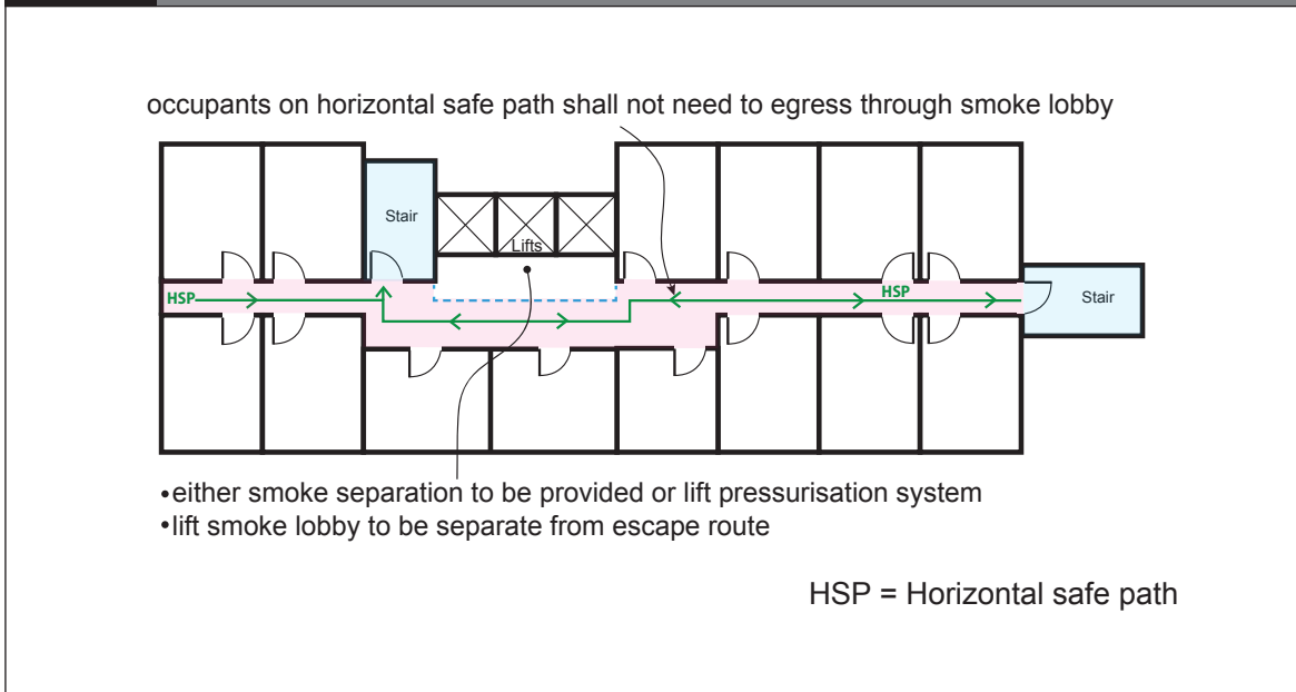
Figure 3.18 Lifts and smoke separations when landing on an unsprinklered horizontal safe path Paragraph 3.10.5
