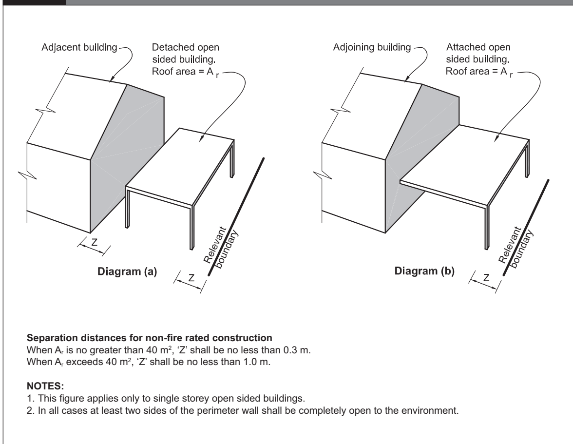
Figure 5.5 Open sided buildings – distance and FRR requirements Paragraph 5.6.6
