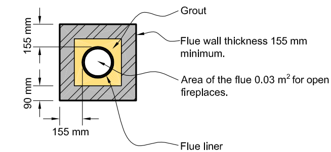
(a) With flue liner
