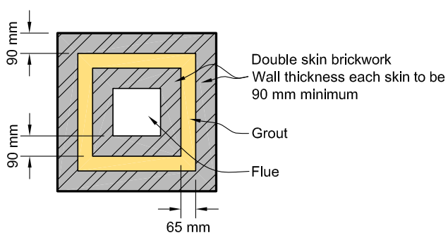
(b) Without flue liner
