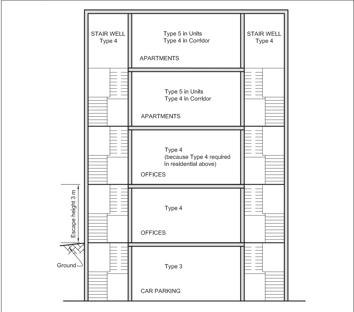
Figure 2.2 Fire safety systems throughout a building Paragraph 2.2.5
